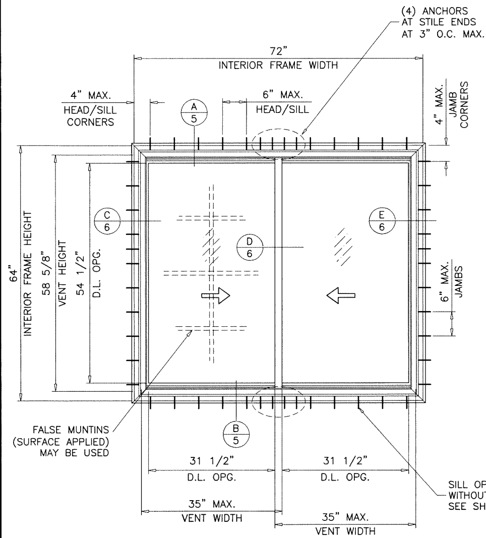
FLANGE FRAMES
