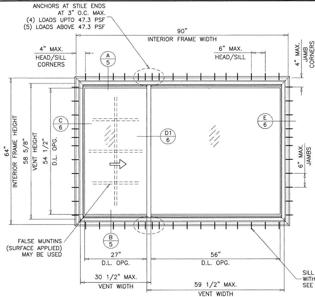
FLANGE FRAMES
