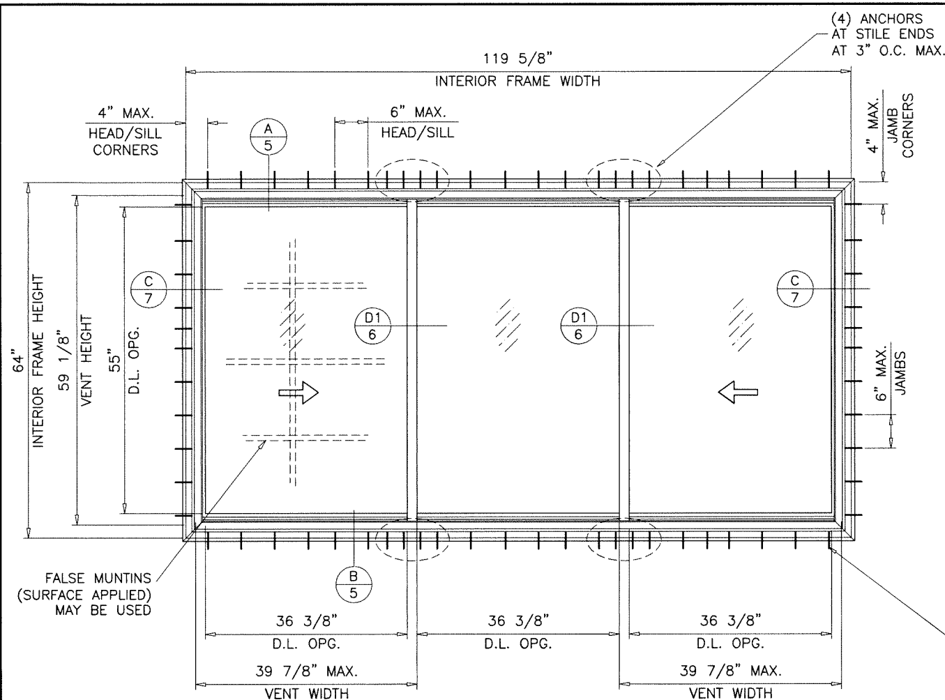
FLANGE FRAMES
