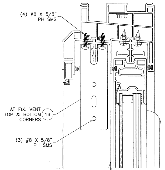
FIX. VENT TOP/BOTTOM CONNECTION
