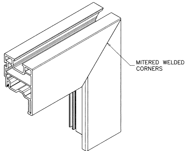
VENT CORNERS
