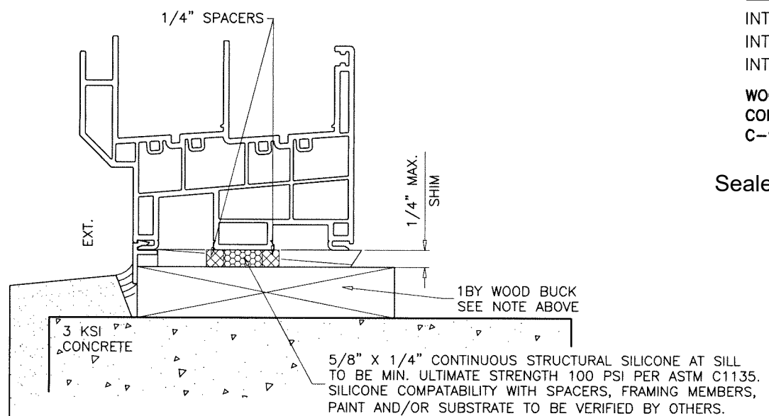
SILL OPTION WITHOUT FRAME ANCHORS
